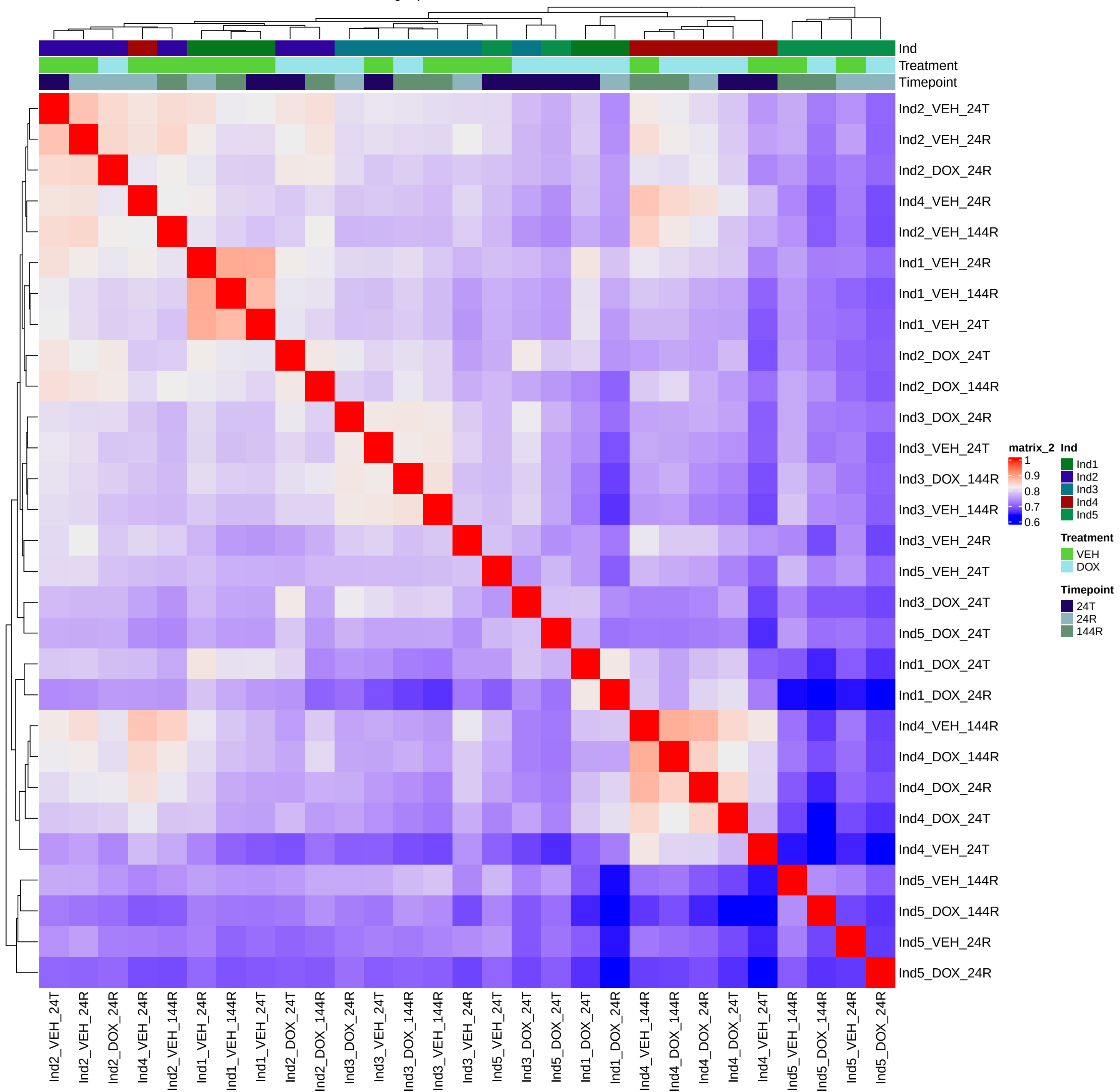
Unfiltered log2cpm H3K27me3 with no removal
